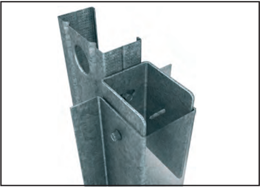
VERTICAL METHOD TO STEEL STUD FRAMING
