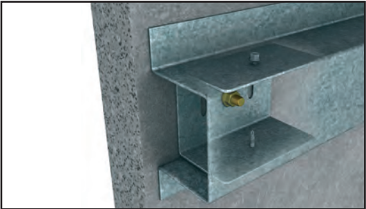
CLEAT TO CONCRETE
